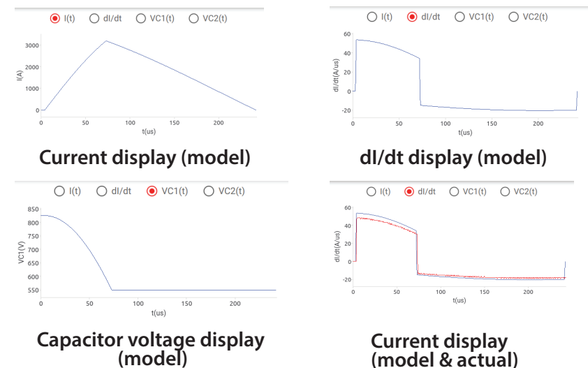
Fig. 2-18: Pulse waveform display
